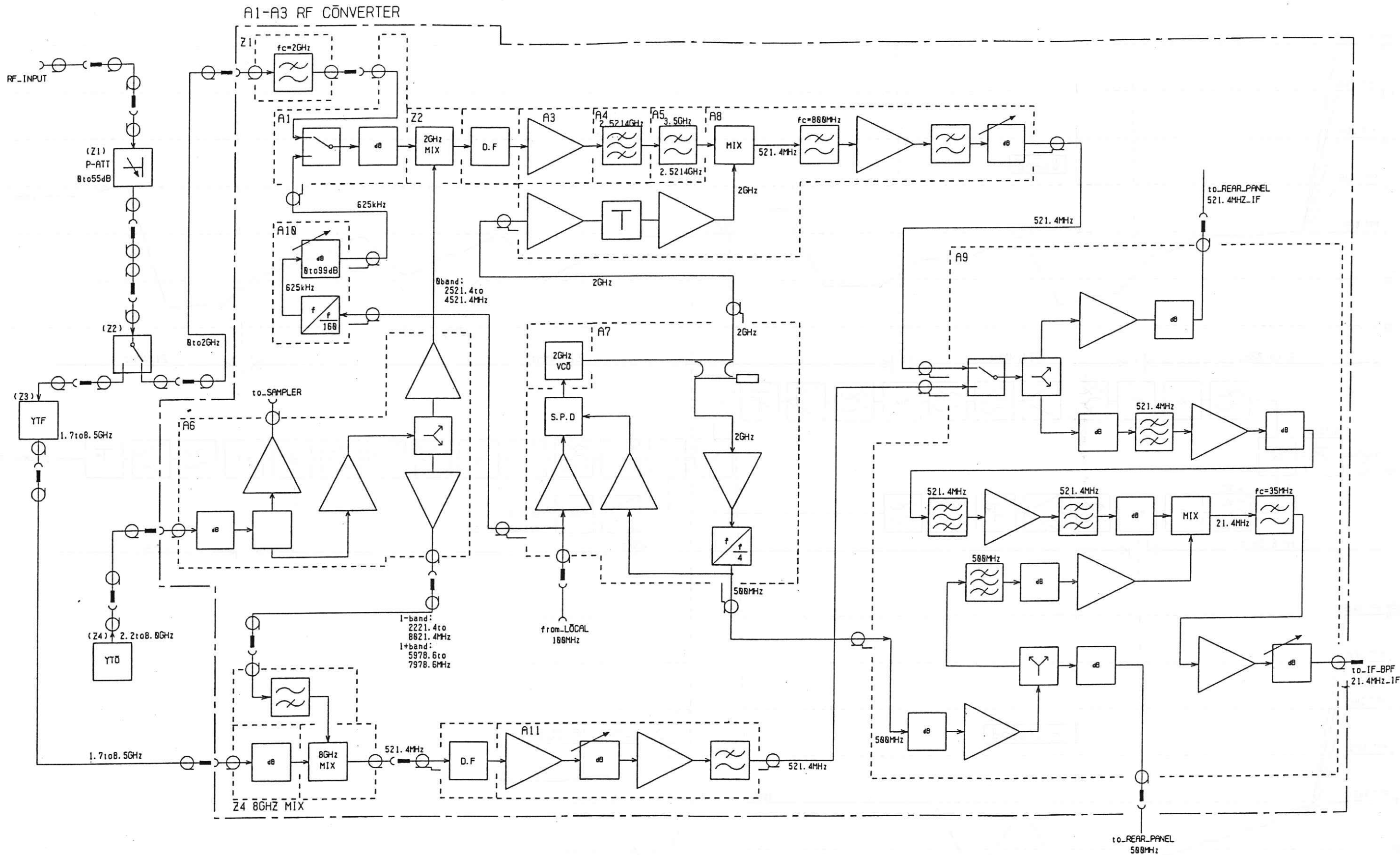
Fig. 2-2 A1-A3 RF CONVERTER Block Diagram
