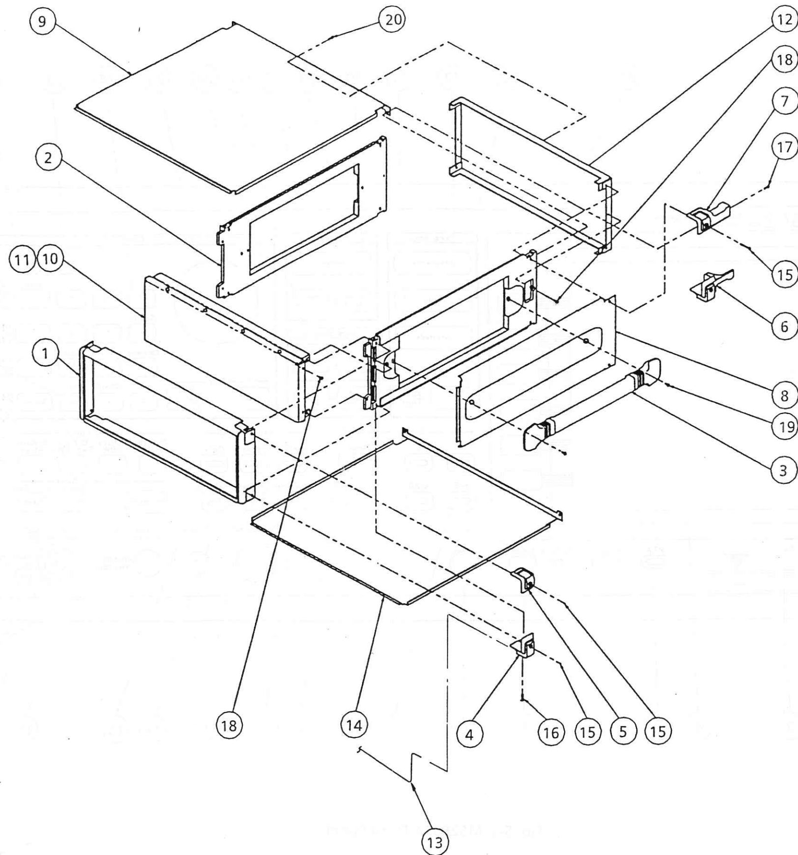
Fig. 5-1 Cabinet Assembly
